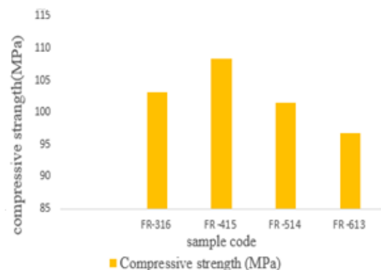
Fig 6. Graphical depiction of compressive strength for a composite sample
