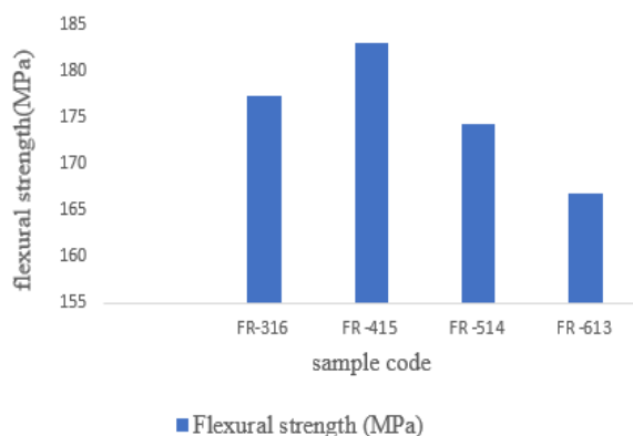
Fig 5. Graphical depiction of flexural strength for a composite sample
