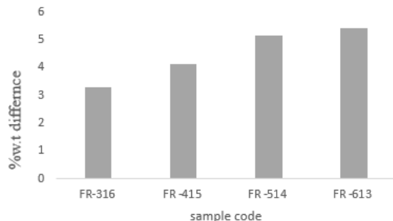
Fig 7. Graphical depiction for water absorption in composite sample
